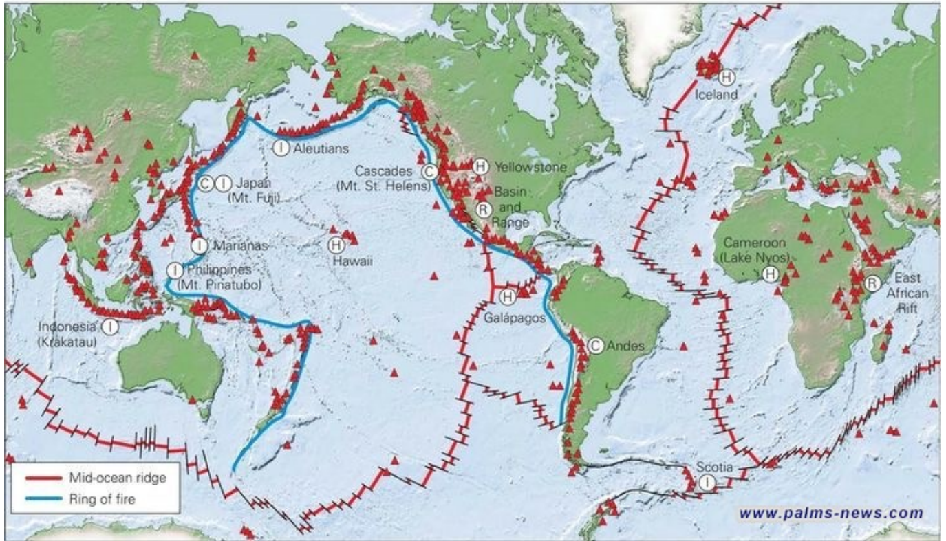
Ⓘ = Island arc
