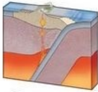
Ⓘ = Island arc
