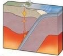
Ⓒ = Continental arc
