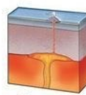
Ⓗ = Hot spot
